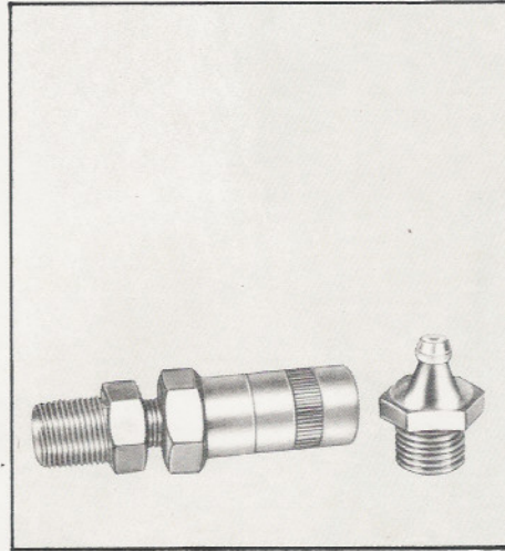
HYDRAULIC CONNECTOR CAT. NO. 6304-B/101 For Hydraulic type Grease Nipple.
