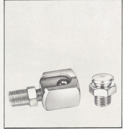
TAT HEXAGON HOOK-ON CONNECTOR CAT. NO. 42030/101 For 'TAT' Hexagon and Industrial Round Head Nipple.
